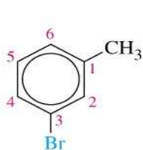
3-Bromotoluene ( m -bromotoluene)
