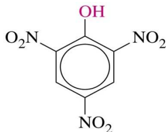
2,4,6-Trinitrophenol (picric acid)
