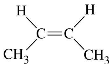
(a) cis -2-Butene
