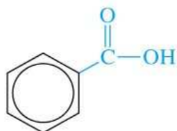
Benzoic acid (an aromatic acid)
