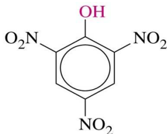
2,4,6-Trinitrophenol (picric acid)
