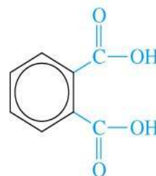
o-Phthalic acid (an aromatic dicarboxylic acid)
