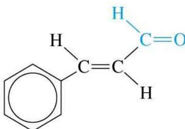
Cinnamaldehyde (cinnamon)
