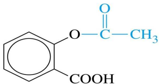
Acetylsalicylic acid (aspirin)
