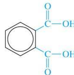
o -Phthalic acid (an aromatic dicarboxylic acid)
