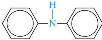
Diphenylamine (a secondary amine)
