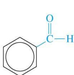
Benzaldehyde (almonds)
