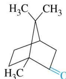
Camphor (obtained from camphor tree)
