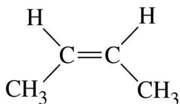
(a) cis -2-Butene
