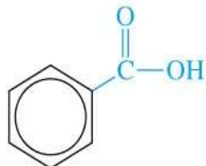
Benzoic acid (an aromatic acid)
